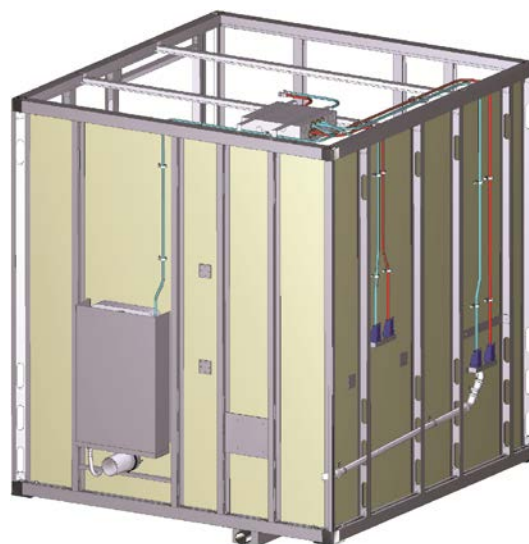
Fig. 2 External view; Bathsystem Superlight Bathroom Pod.
